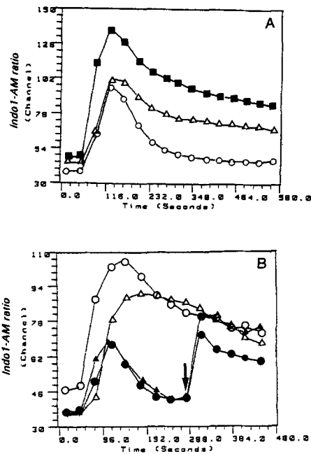
Figure 3. Ca^{2+} mobilization after CD3 and CD50 co-cross-linking, and after CD50 and CD3 individual cross-linking, in absence of extracellular Ca^{2+} . (A) Additional effect of the costimulation with anti-CD3 (Cris-7) and anti-CD50 on Jurkat cell line. Cris-7 (O-O), 1 ng/ml; 152-2D11 ( \Delta - \Delta ), 50 \mu g/ml; and 152-2D11 + Cris-7 ( \blacksquare - \blacksquare ), 50 \mu g/ml + 1 ng/ml; cross-linked at 50 s with 10 \mu g/ml of GAM. (B) Jurkat cells were stimulated by cross-linking CD3 and CD50 at 50 s in an INDO-1 buffer C with 100 mM EGTA and without CaCl_2 and or with 10 \mu M CaCl_2 was added at 300 s (arrow). Stimulations in presence of extracellular Ca^{2+} are also presented. Cris-7, 1 ng/ml, with (O-O) and without ( \bullet - \bullet ) extracellular Ca^{2+} , and 152-2D11, 50 \mu g/ml, with ( \Delta - \Delta ) and without ( \blacktriangle - \blacktriangle ) extracellular Ca^{2+} , cross-linked at 50 s with 10 \mu g/ml of GAM.
